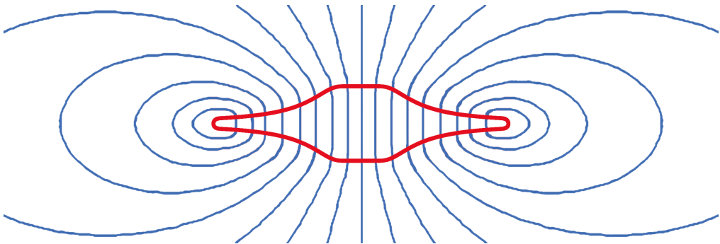
Fig. 25 – Parallel magnetic field lines inside an electrostatically charged discock object rotating around its z -axis (cross-section).
